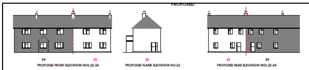
Figure 3 - proposed elevations
